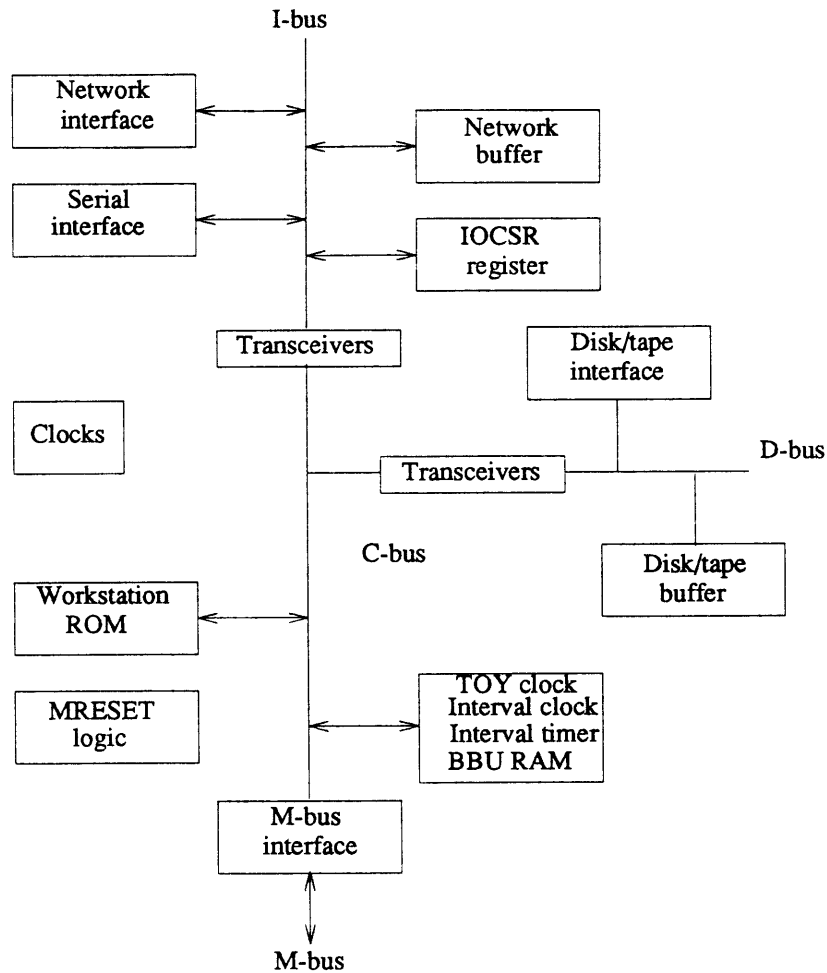
Figure 7-1: Firefox Workstation I/O Module Block Diagram
